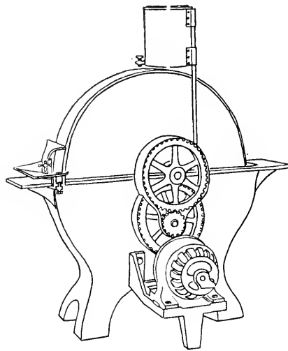
FIG. 218. MOTOR DRIVEN GRINDSTONE.
